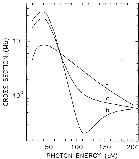
FIG. 6. Atomic subshell photoionization cross sections as a function of photon energy for Mn 3 d (a) and Pd 4 d (b) orbitals. Data are compiled from Ref. 57. Curve (c) is the weighted average of curves (a) and (b) with the weights corresponding to the Mn and Pd concentrations in \text{Al}_{70}\text{Pd}_{20}\text{Mn}_{10} . Note the logarithmic scale on the ordinate axis.
