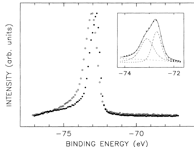
FIG. 10. Al 2p photoemission spectra of the Al metal (●) and i\text{-Al}_{70}\text{Pd}_{20}\text{Mn}_{10} alloy (○). The spectra were normalized to give a constant height between the maximum and minimum recorded count. The inset shows the fit of the Al 2p spectrum of the Al metal with two component Voigt lines, which are also shown, corresponding to Al 2p_{1/2} and 2p_{3/2} core levels.
