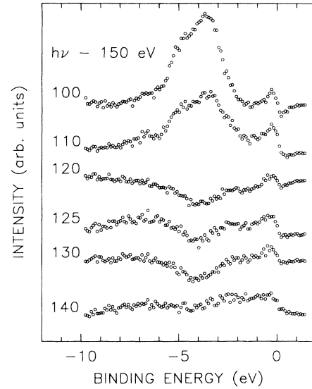
FIG. 9. Difference spectra obtained from the PES spectra in Fig. 8 by subtracting from them the spectrum measured at h\nu=150 eV. The numbers on the left side of each difference spectrum indicates the photon energy of the spectrum from which the h\nu=150 eV spectrum was subtracted.
