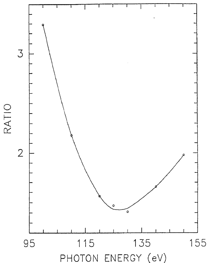
Fig. 3. Intensity ratio of the two features in Fig. 2 at the binding energies -3.6 and -0.7 eV as a function of photon energy. The solid line is a guide for the eye.
