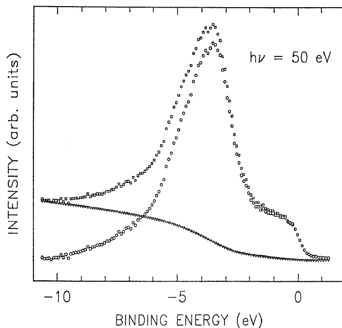
Fig.1 Effect of the secondary-electron contribution on the valence-band spectrum of i\text{-Al}_{70}\text{Pd}_{20}\text{Mn}_{10} measured with a photon energy h\nu = 50 eV. (□) - original spectrum, (▽) - secondary-electron contribution to the analyzer- and flux-corrected original spectrum, (○) - resultant spectrum after subtraction of the secondary - electron contribution.
