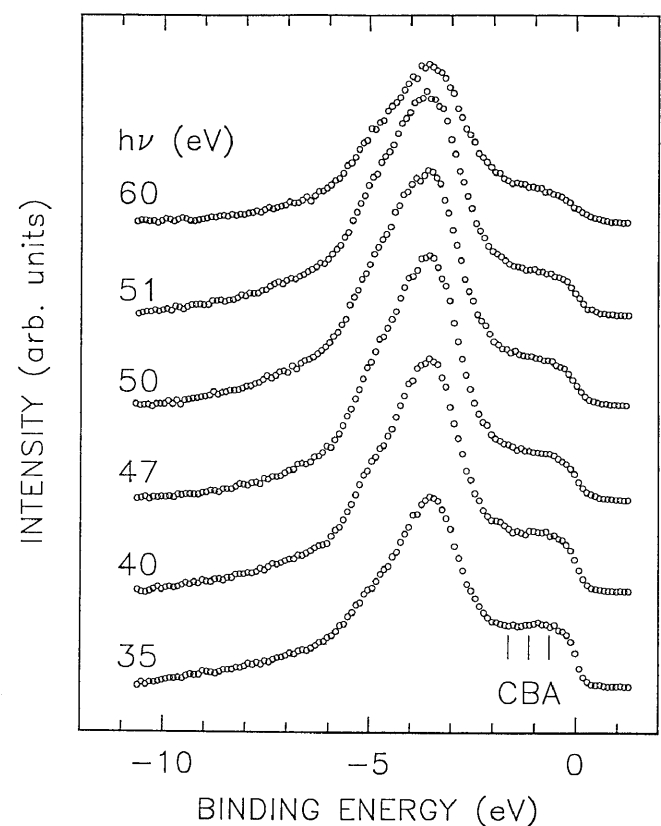
Fig. 4 Valence-band spectra of i\text{-Al}_{70}\text{Pd}_{20}\text{Mn}_{10} for different photon energies h\nu around the Mn 3p \rightarrow 3d transition. A, B, and C identify features for which CIS spectra were measured (Fig. 5).
