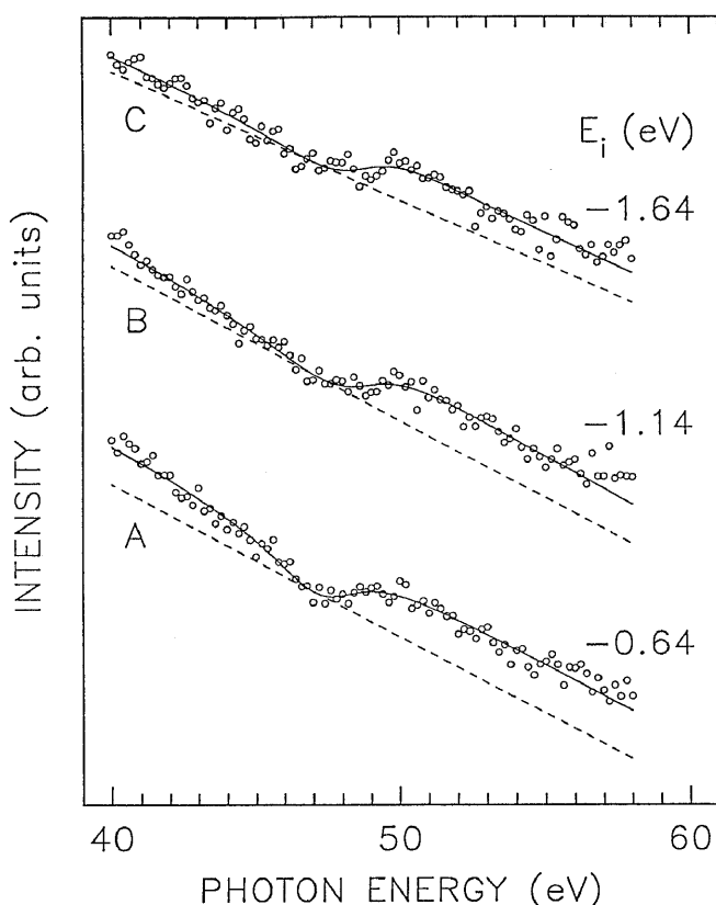
Fig. 5 Constant-initial-state (CIS) spectra for the valence-band features A, B, and C in Fig. 4 that are identified here by the same letters and by their corresponding initial energies E_i . The solid line is a fit to the Fano profile and a linear background (shown by a broken line), as described in the text.
