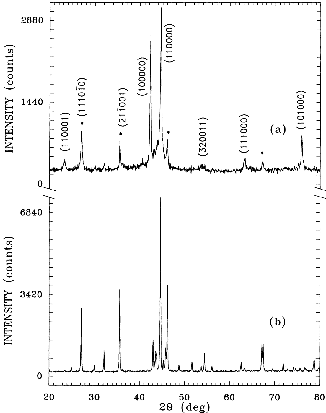
FIG. 2. X-ray-diffraction patterns obtained with \text{Cu } K\alpha_1 radiation of icosahedral \text{Al}_{40}\text{Cu}_{9.94}\text{Fe}_{0.06}\text{Ge}_{25}\text{Mn}_{25} (a) in an as-quenched state and (b) heated up to 798 K at a rate of 20 \text{ K min}^{-1} in a DTA analyzer. The centers of the symbols * in (a) correspond (in an increasing 2\theta sequence) to the positions of (101), (111), and (200) lines, and the average position of narrowly separated (203) and (220) lines of \text{AlGeMn}_{0.995}\text{Fe}_{0.005} from Fig. 1(b).
