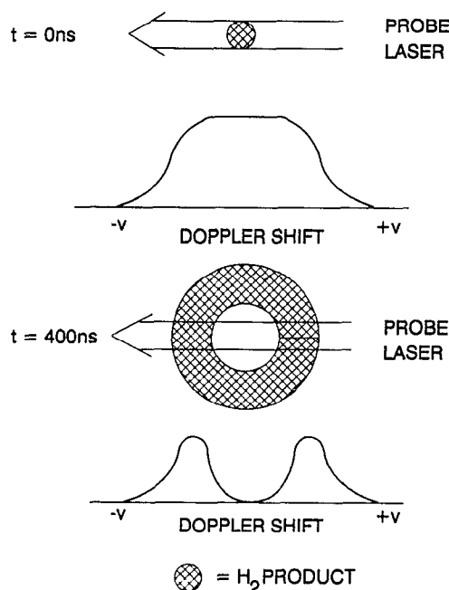
FIG. 10. Pictorial representation of the time delay effect used in velocity aligned Doppler spectroscopy (VADS). Shown are (top) probe beam/ \text{H}_2 product overlap and expected line profile at zero time delay and (bottom) probe beam/ \text{H}_2 product overlap and expected line profile at a long time delay (400 ns). The cross hatched areas represent the spatial distribution of the \text{H}_2 dissociated from \text{C}_2\text{H}_4 .
