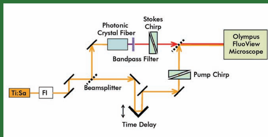
Figure 2. A simple CARS microscope. A beamsplitter splits pulses from an isolated femto-second Ti:sapphire laser. Half goes to a photonic crystal fiber to generate the Stokes pulses, followed by a bandpass filter, before being recombined on a dichroic mirror.
