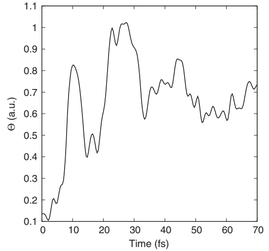
FIG. 4. Time evolution of the charge transfer metric \Theta calculated using the results of AIMS simulations of ethylene excited to the \pi\pi^* state. The large, transient charge separations occurs when the wave packet encounters the Tw-Py CI and is responsible for the distinguishability of the two C atoms at the CI.
