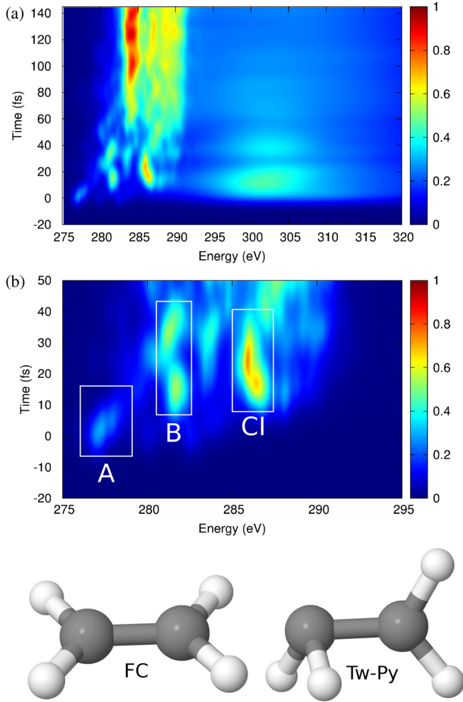
FIG. 2. The TRXAS spectrum calculated from AIMS simulations of ethylene excited to its \pi\pi^* state. (a) The full spectrum showing both the pre-edge and postedge continuum absorption. (b) The pre-edge part of the spectrum at short times and the relevant peak assignments. The features labeled A, B, and CI are directly related to the associated dynamical features shown in Fig. 1. The FC (A) and Tw-Py intersection (CI) geometries are shown below. The color map represents the relative probability of absorption.
