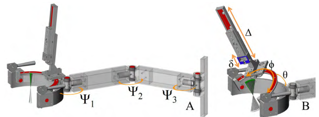
FIGURE 2. CAD models of the articulated 6-DOF PALOMINO positioning-arm. (A) demonstrates the complete 6-DOF articulating PALOMINO positioning-arm in an upright resting position. Each mechanical component providing a DOF is marked red. The three pin joints of the articulating arm \psi_1 , \psi_2 , and \psi_3 provide redundant 3-DOF planar positioning of the PALOMINO scan-head. (B) demonstrates the 3-DOFs of the end-effector wrist comprised of a linear track mounted to a ring carriage for controlling the scan head's orientation and approach. \theta , \phi , and \Delta (including \delta ) represent the spatial positioning motion of the wrist, the rotation around a common centre along the ring, and the linear travel of the track to position the PALOMINO scan-head, respectively. The workspaces of the GRIN needle objective, for seven discrete positions of \theta between 0 and 30°, are depicted by the green conical half-shells. The cone height is determined by the location \Delta of the instrument mounting platform positioned along the linear track. The shell's radius is determined by the carriage's location \phi on the semicircular rail. Pivoting around these end-effector pins, the arch can rotate approximately 270° about its radial axis \theta . The intersection of the conical shell workspaces is the location of the insertion point of the GRIN needle.
