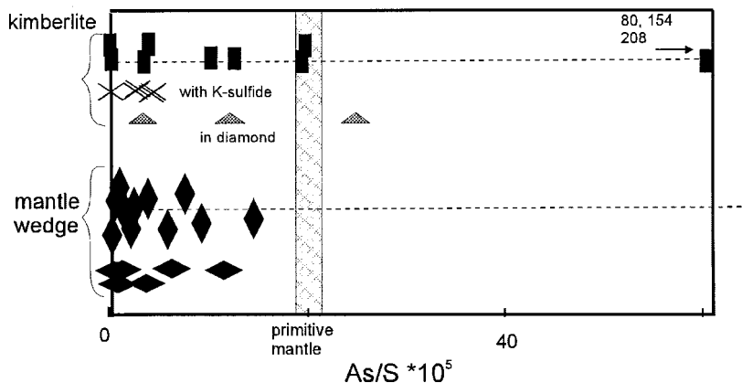
FIG. 3. Range of As/S values in sulfide grains. Symbols same as in Figure 2. Three sulfides grains with high As/S plot outside the range of the diagram and are indicated by an arrow.
