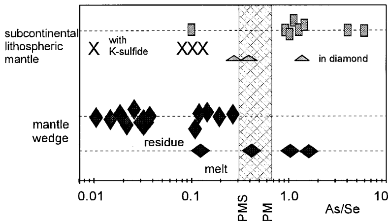
FIG. 6. Range of As/Se values of all sulfide grains sampled. Symbols same as in Figure 5. The values of As/Se in primitive mantle (PM) and primitive mantle sulfide (PMS) are listed in Table 3.
