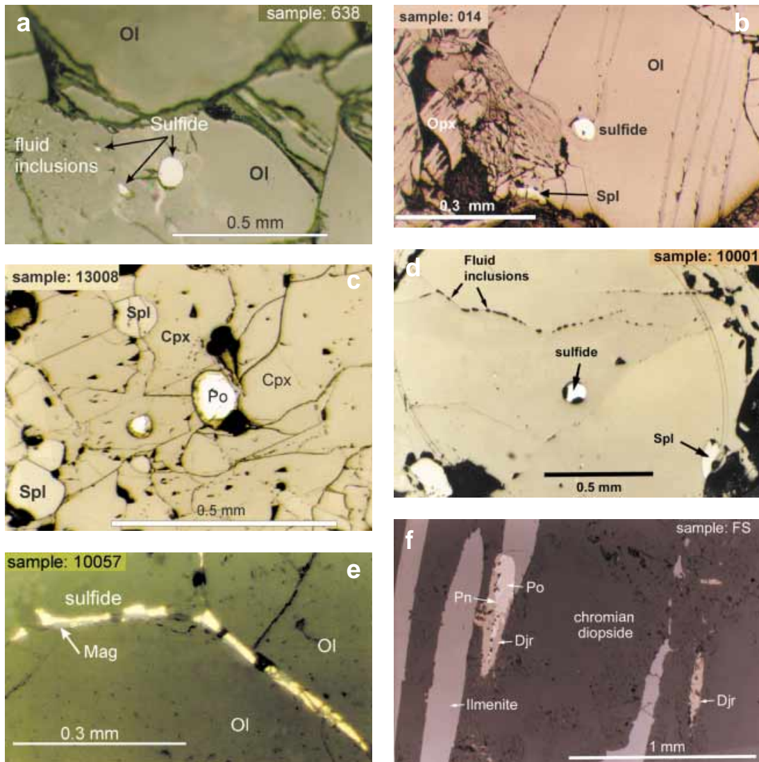
FIG. 1. Photomicrographs showing the mode of occurrence of sulfide grains, taken under reflected light. a. Spherical sulfide grain enclosed in olivine (Ol) in harzburgite (sample 638) from Ichinomegata, Japan. The sulfide is predominantly pentlandite. The olivine ( \text{Fo}_{90.0} ) contains abundant fluid inclusions. b. Sulfide grain enclosed in olivine ( \text{Fo}_{83.4} ) in spinel hercynite (sample 014) from Ichinomegata, Japan. The sulfide is pentlandite and pyrrhotite. Ol: olivine, Opx: orthopyroxene, Spl: chromian spinel. c. Globular sulfide grain along grain boundaries of clinopyroxene (Cpx) and olivine (Ol) in spinel pyroxenite (13008) from Nunivak Island, Alaska. Cpx: clinopyroxene, Spl: spinel, Po: pyrrhotite. d. Spherical grain of sulfide in orthopyroxene in hercynite (sample 10001) from Nunivak Island, Alaska. The large circle is engraved for analytical purposes. e. Veinlets containing primary sulfide along grain boundaries of olivine (Ol) in spinel hercynite (sample 10057) from Nunivak Island, Alaska. The veinlet contains pyrrhotite and exsolution products of pentlandite and magnetite (Mag). f. Sulfide phases and ilmenite inclusions oriented within diopside megacryst in kimberlite from Frank Smith mine, South Africa (sample FS). Djf: djerfisherite, Po: pyrrhotite, Pn: pentlandite. Pentlandite, a product of exsolution of monosulfide solid-solution, rims the sulfide phase. The diopside host contains high Mg [atomic \text{Mg}/(\text{Mg} + \text{Fe}) = 0.87 ], Na (1.68–1.78 wt% \text{Na}_2\text{O} ), Cr (0.33–0.56 wt% \text{Cr}_2\text{O}_3 ) and Ni (390–890 ppm).
