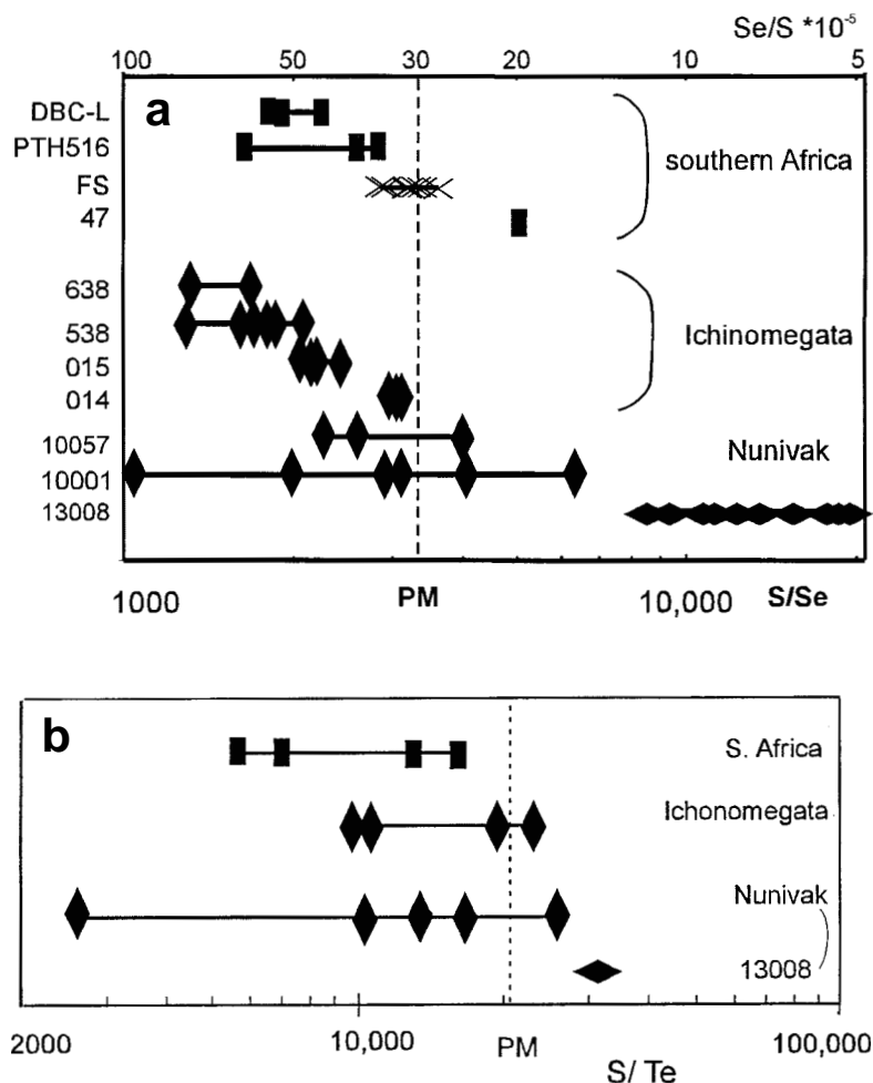
FIG. 2. a. Range of S/Se values in all samples. The ratio of primitive mantle (PM) calculated from the values given by McDonough & Sun (1995) is shown by the dashed line. b. Range of S/Te values in all samples. Solid diamonds: samples from mantle wedges at Nunivak and Ichinomegata. Tall diamonds represent residues (lherzolite and harzburgite) and short tabular diamonds represent garnet clinopyroxenite (solidified melt in the mantle) from Nunivak Island. \times : Sulfide associated with potassium sulfides in diopside megacryst in kimberlite. Squares: peridotite nodules in kimberlite.
