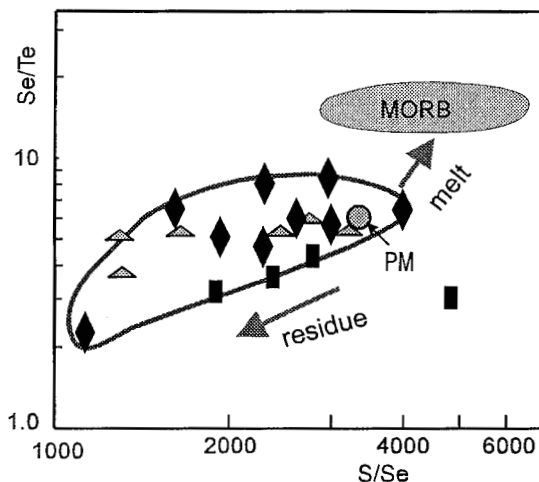
FIG. 5. S/Se and Se/Te values of sulfides from mantle rocks. Symbols same as those in Figure 2. The data on sulfides enclosed by diamonds in peridotitic assemblages with no apparent fractures (shown as solid triangles) are from Bulanova et al. (1996). Data on mid-ocean-ridge basalts (MORB) from Hertogen et al. (1980), Hamlyn & Keays (1986) and Peach et al. (1990).
