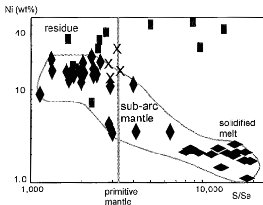
FIG. 4. Concentrations of Ni and S/Se values in all samples. Primitive mantle value is from McDonough & Sun (1995).
