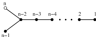
Fig. 1. The Dynkin graph of type D_n . We represent the n th vertex by an open dot to distinguish it from the (n - 1) st vertex.
