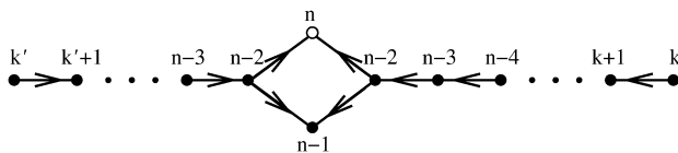
Fig. 6. The string representing (\tilde{\mathbf{V}}(k', k), \tilde{x}(k', k)) , 1 \leq k' < k \leq n - 2 .
