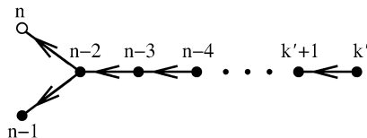
Fig. 5. The (forked) string representing (\mathbf{V}(k', n + 1), x(k', n + 1)) , 1 \leq k' \leq n - 2 .
