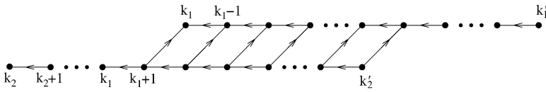
Fig. 7. If x_{h_{i,i-1}}(e_i^2) \neq 0 for some i , the commutativity of the above diagram forces k'_2 > k'_1 and k_2 > k_1 . The vertices in the upper (respectively lower) string represent the basis vectors defining the representation (\mathbf{V}(k'_1, k_1), x(k'_1, k_1)) (respectively (\mathbf{V}(k'_2, k_2), x(k'_2, k_2)) ). A vertex labeled i represents e_i^j \in \mathbf{V}_i ( j = 1, 2 ). The arrows indicate the action of the obvious component of x .
