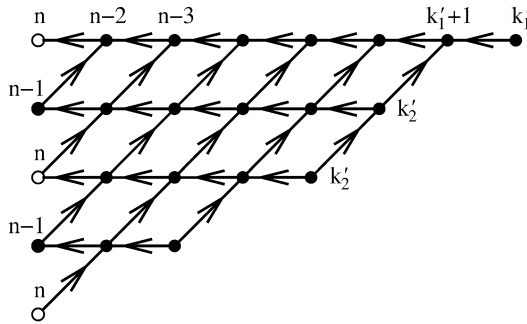
Fig. 9. The irreducible components of \bigcup_{\mathbf{v}} \mathcal{L}(\mathbf{v}, \mathbf{w}^n) are enumerated by Young diagrams.
