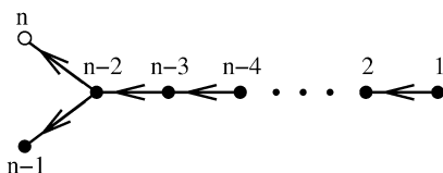
Fig. 2. The quiver (oriented graph) of type D_n .
