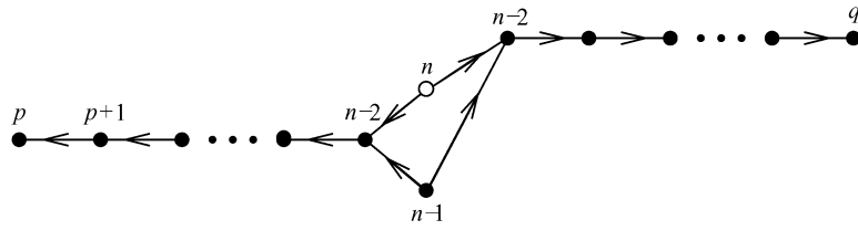
Figure 9. The string corresponding to an entry \overline{n-1} in the p th row in a tableau mapping into the string corresponding to an entry n-1 in the q th row. The second string has been reversed from its usual presentation.
