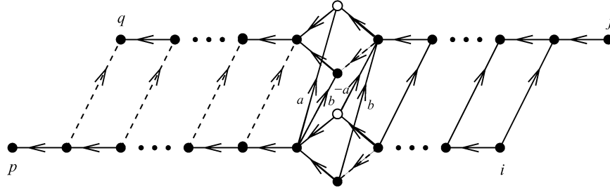
Figure 6. A map from the string corresponding to an entry \bar{i} in the p th row of a tableau into the string corresponding to an entry \bar{j} in the q th row for i, j, p, q \leq n-2 . Unmarked solid and dotted lines indicate a coefficient of 1 and -1 respectively. Otherwise the lines are labelled by the value of the coefficient. These must satisfy a + b = -1 .
