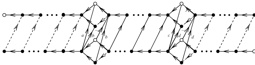
Figure 17. One column mapping into another. We depict the blocks by vertices. Unmarked solid and dotted lines indicate a coefficient of 1 and -1 respectively. Otherwise the lines are labelled by the value of the coefficient. These must satisfy a + b = -1 and c + d = 1 .
