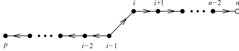
Figure 11. The string corresponding to the entry i in the the p th row of tableau mapping into the string corresponding to the entry \bar{i} in a half box.
