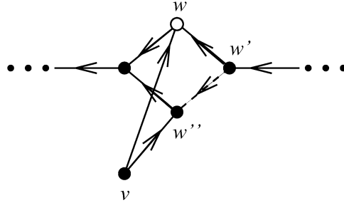
Figure 12. The vector v mapping into the degree n vertex of a string corresponding to an entry \alpha, \alpha \geq n - 2 , in row p, p < n - 1 .
