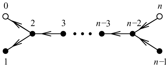
Figure 15. The quiver of type D_n^{(1)} .
