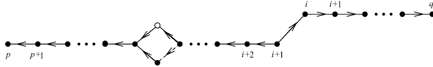
Figure 8. The string corresponding to an entry \overline{i+1} in the p th row of a tableau mapping into the string corresponding to an entry i+1 in the q th row for i \leq n-3 . The second string has been reversed from its usual presentation.
