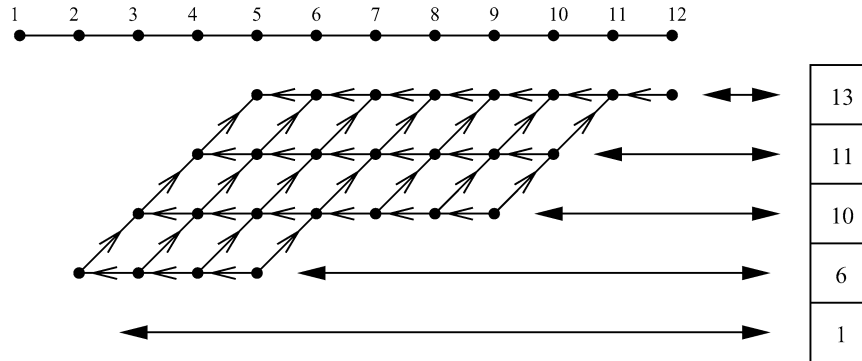
Figure 4. The correspondence between strings/rows in a Maya diagram of charge 5 and the entries in a 5 box column in a Young tableau for the case of A_{12} . The entry is one greater than the degree of the right endpoint of the string/row of the Maya diagram. An empty string/row corresponds to an entry equal to the where the left endpoint of the string would have been. The column of the Young tableau has been inverted to better show the correspondence.
