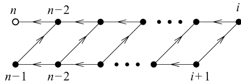
Figure 10. The string corresponding to the entry \overline{i+1} in a half box mapping into the string corresponding to the entry \overline{i} in a half box.
